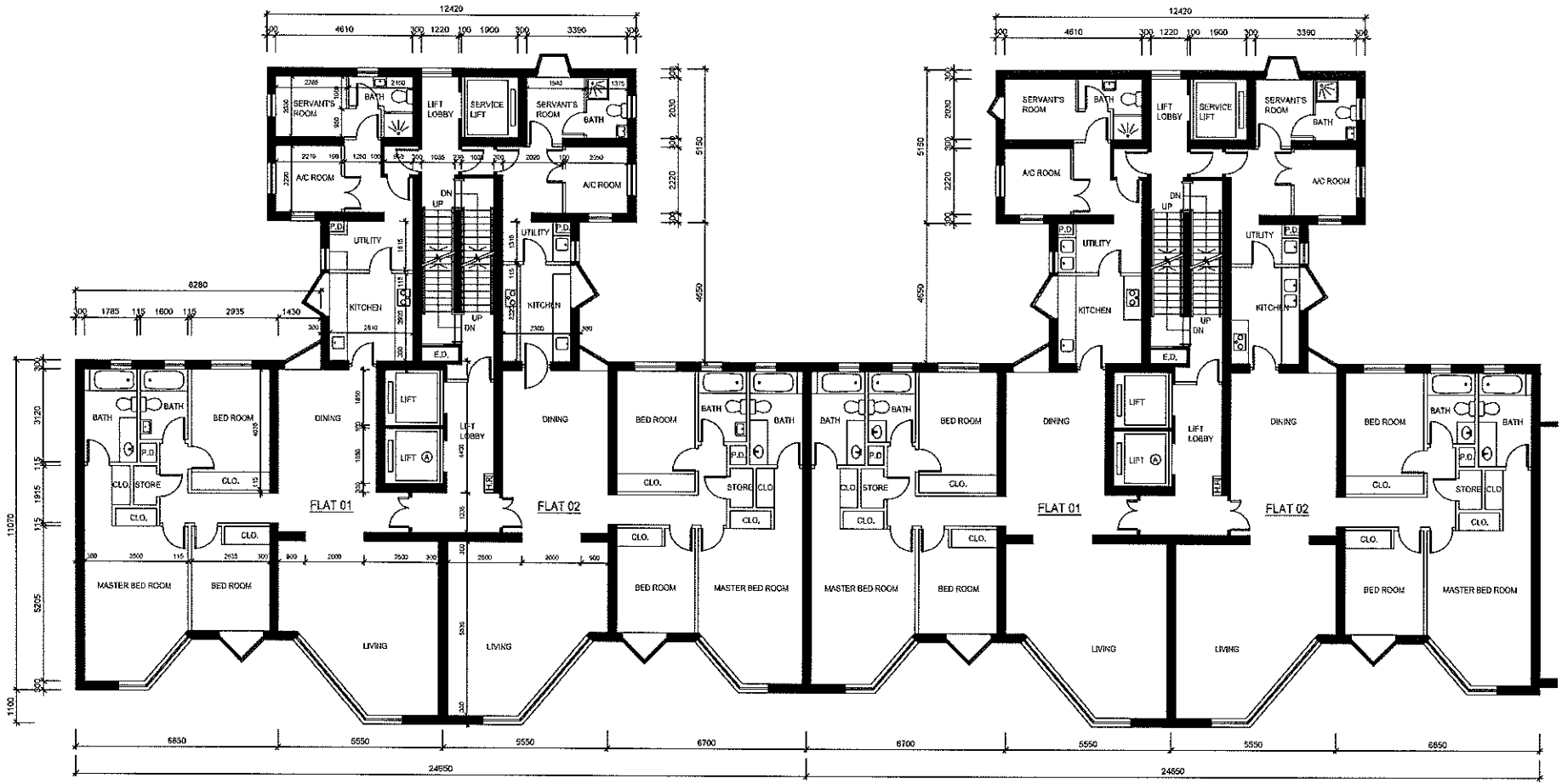
1st TO 31st TYPICAL FLOOR PLAN BAMBOO GROVE (BLOCK 78)
